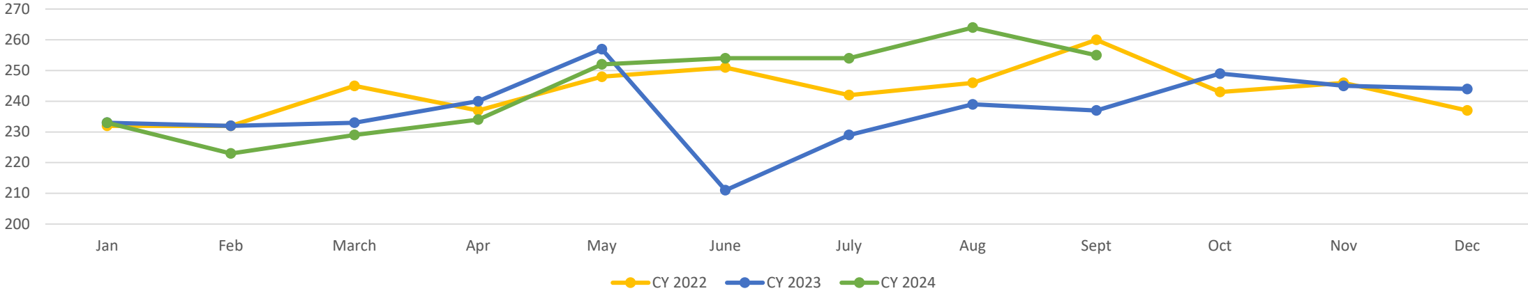
MONTHLY PEAK DEMAND THRU September 30, 2024
