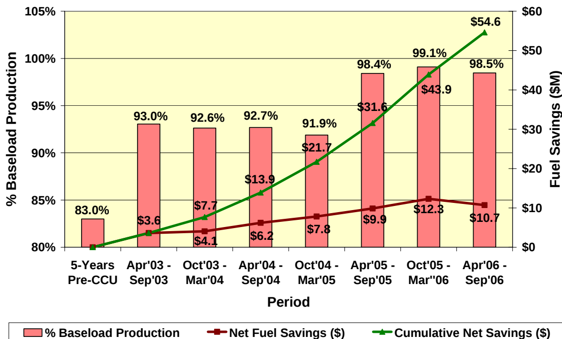
Figure 2, Baseload Production and Fuel Savings by Current Management over Prior Management
